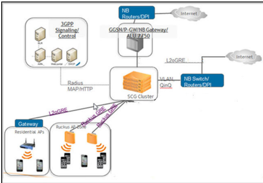
FIGURE 1 Tunneling Interface
